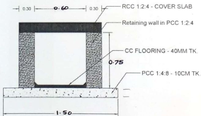
SECTION OF 'U' DRAIN B-TYPE
