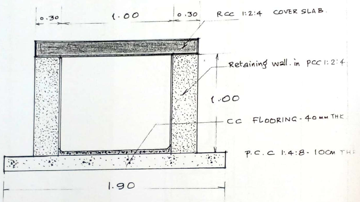
SECTION OF 'U' DRAIN C-TYPE
