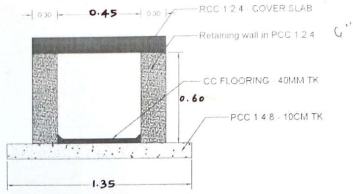
SECTION OF 'U' DRAIN A-TYPE
