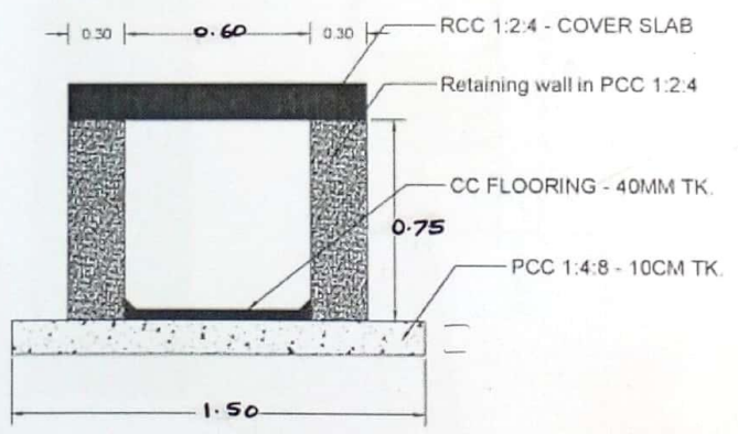
SECTION OF 'U' DRAIN B-TYPE
